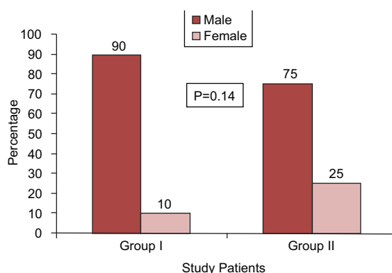
Fig.-1: Sex distribution of the study patients (N=80).
